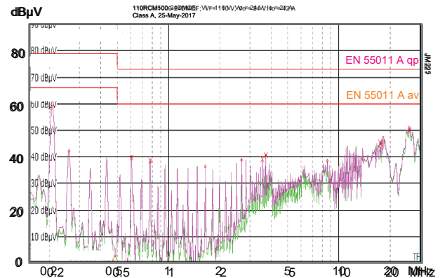
Fig. 9b 110RCM1000-24: Typ. conducted disturbances at the input ( V_i = 110 V, I_{i\text{nom}} , resistive load, quasi peak and average).
