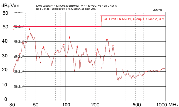
Fig. 10a 110RCM500-24: Typ. radiated disturbances in 3 m distance ( V_i = 110 V, I_{i\text{nom}} , resistive load, quasi peak).
