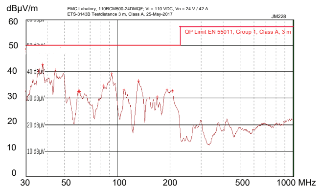
Fig. 10b 110RCM1000-24: Typ. radiated disturbances in 3 m distance ( V_i = 110 V, I_{i\text{nom}} , resistive load, quasi peak).
