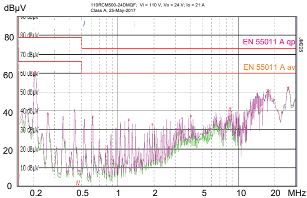
Fig. 9a 110RCM500-24: Typ. conducted disturbances at the input ( V_i = 110 V, I_{i\text{nom}} , resistive load, quasi peak and average).
