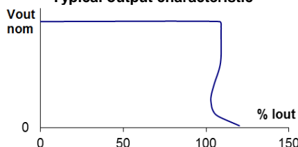
Typical output characteristic
