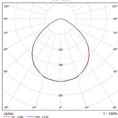
COMPACT LED EVO N 42W 840 PRM II CLASS
