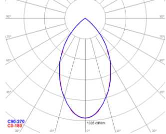
DRAG-M-55_140W_4000K
