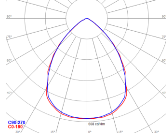
DRAG-M-85_140W_4000K
