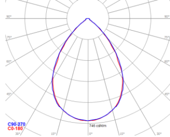
DRAG-M-75_140W_4000K
